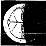
One drawing of the Venusian radial-spoke system
